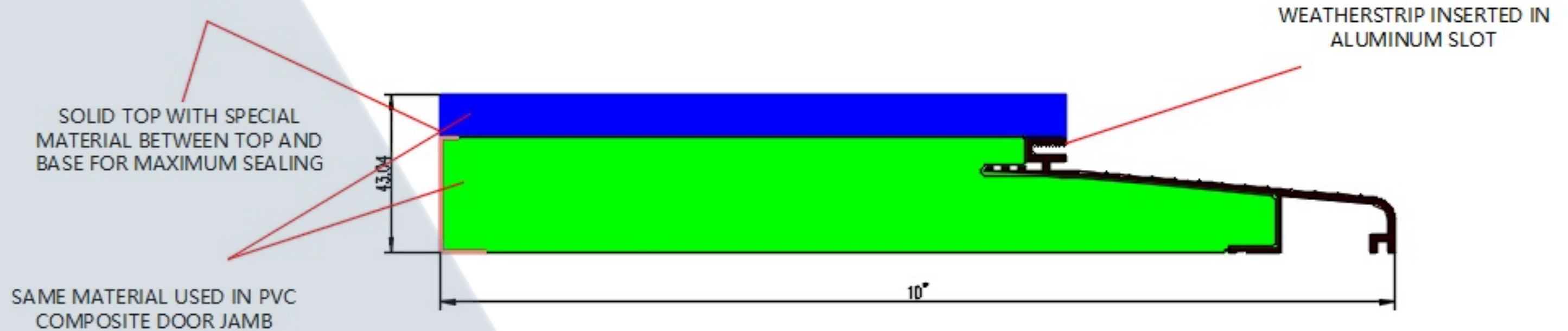
1000-OUT-VINYL TOP FOR 8 7/8" DOOR JAMB
